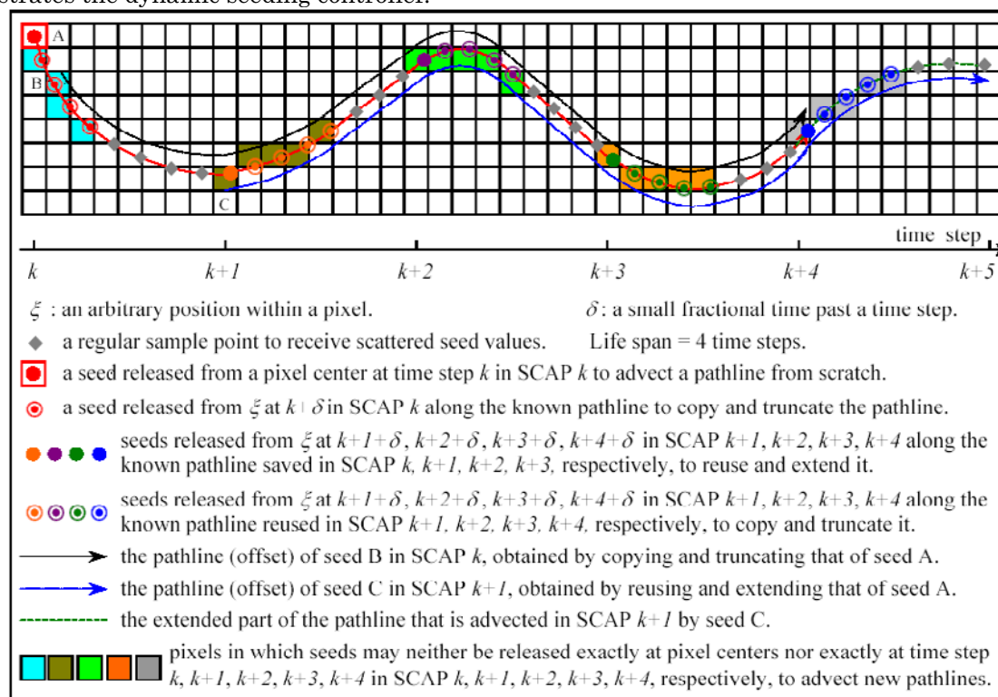
Fig. 2. The flow-driven seeding strategy. Given the temporal and spatial seeding flexibilities, seeds released along a known pathline can copy and truncate in the same SCAP, as well as reuse and extend between consecutive SCAPs, the pathline for fast value scattering.
