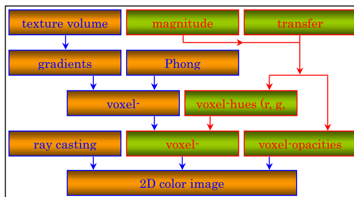
Fig. 5. Our pipeline for rendering 3D AUFLIC textures using a magnitude-based transfer function.
